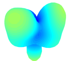
Cx-Pol Gain
